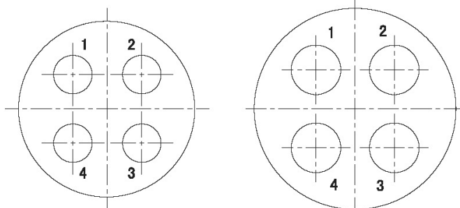
YLD-2404 (4- \phi 7) YLD-3204 (4- \phi 9)
