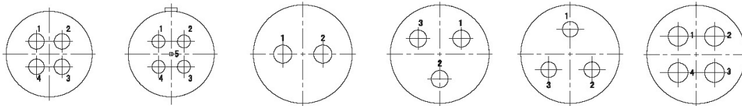
TYLD-1204 (4- \phi 2.5) YLD-1205 (4- \phi 2.5, 1- \phi 1) YLD-1402 (2- \phi 3.5) YLD-1403 (3- \phi 3) YLD-1403a (3- \phi 3) TYLD-1404 (4- \phi 3)
