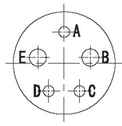
YL-0605 (2- \phi 1.02, 3- \phi 0.76)
