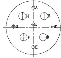
YL-1409 (5- \phi 1.02, 4- \phi 2.39)
