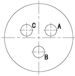
YL-1203a (3- \phi 1.59)
