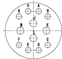
YL-1412 (4- \phi 1.59, 8- \phi 1.02)
