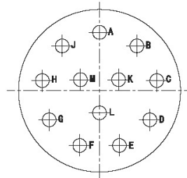
YL-2212 (12- \phi 2.39)
