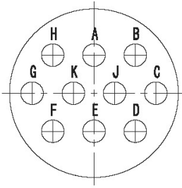
YL-1210 (10- \phi 1.02)
