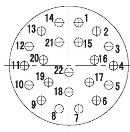
YL-1222 (22- \phi 0.76)
