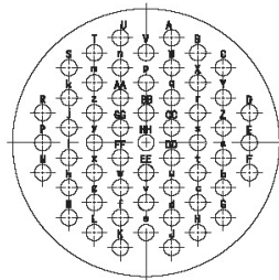
YL-2255 (55- \phi 1.02)
