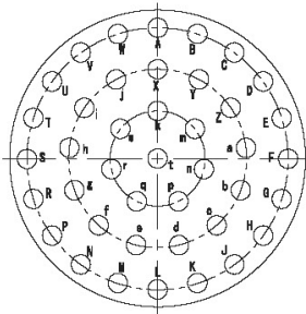
YL-2041 (41- \phi 1.02)
