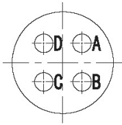
YL-0604 (4- \phi 0.76)
